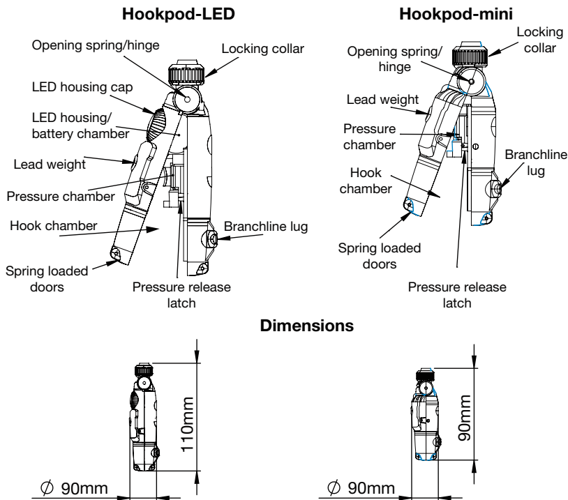
Fig. 1. Relative size and features of the Hookpod_LED and Hookpod-mini
